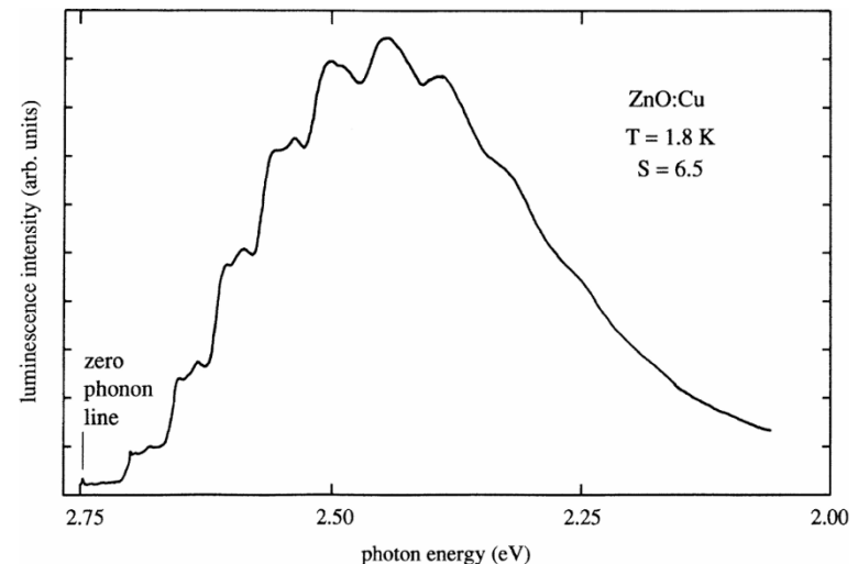
The photoluminescence spectrum of deep centers in ZnO:Cu
