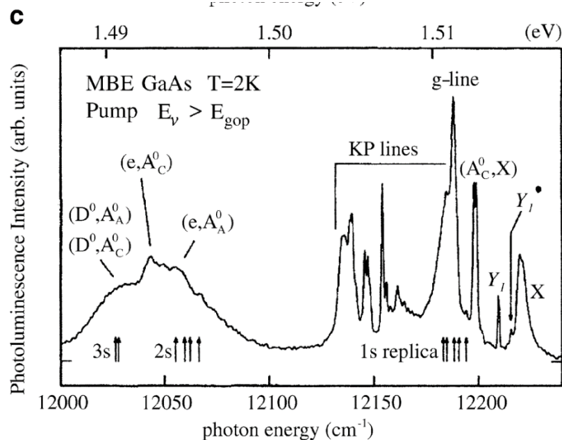
Fig. 14.2 Low-temperature and low-excitation luminescence spectra of ZnO (a) of two differently grown ZnSe samples (solid line: MBE growth with element sources, dashed line: with a compound source) (b) and of GaAs (c)
